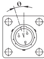
Alternate position of insert with socket contacts (θ counterclockwise)
