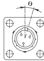
Alternate position of insert with pin contacts (θ clockwise)
