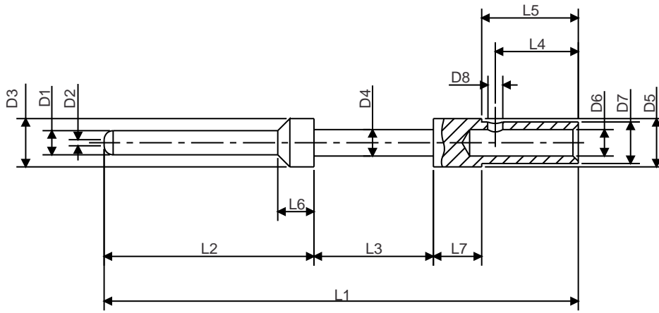
16 & 12 Size Pin Contact (Crimp)
