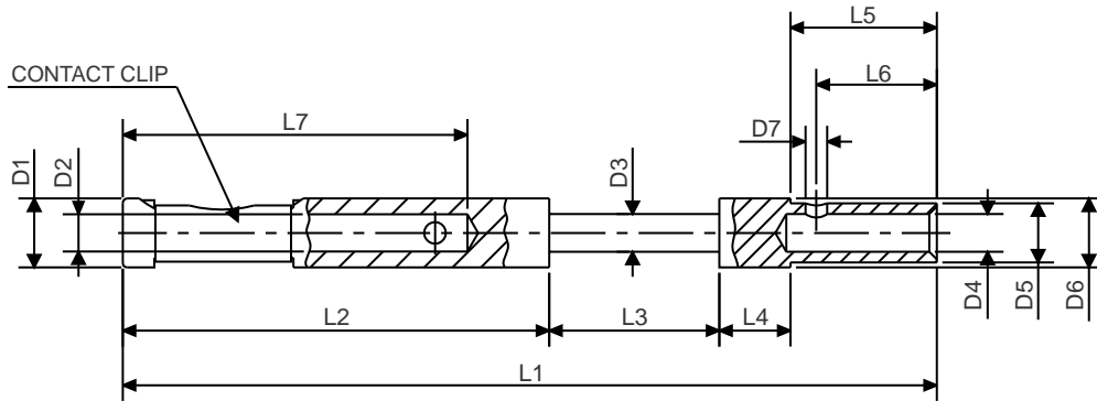
16 & 12 Size Socket Contact
