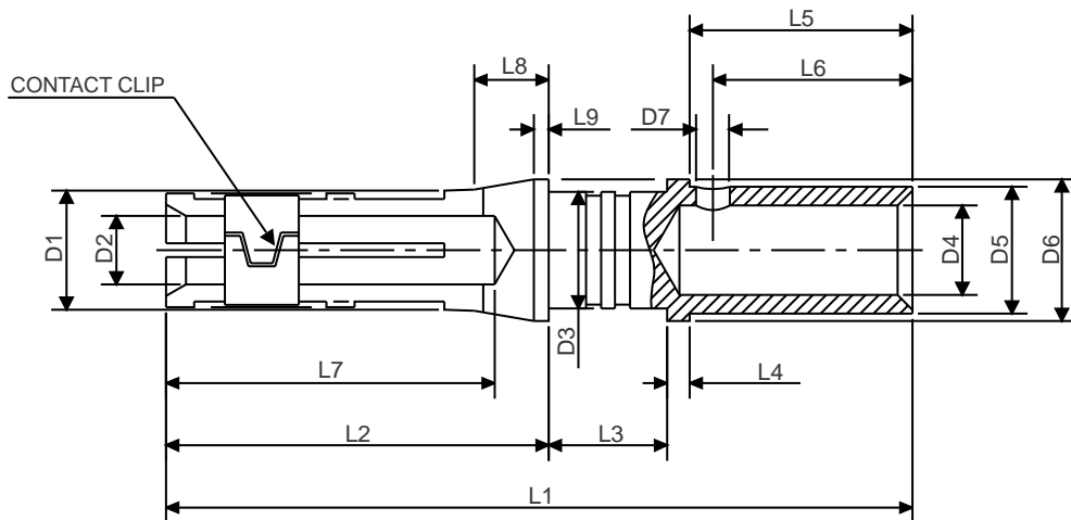
8, 4 & 0 Size Socket Contact
