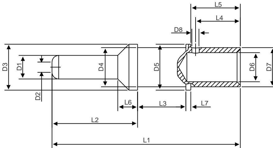
8, 4 & 0 Size Pin Contact (Crimp)
